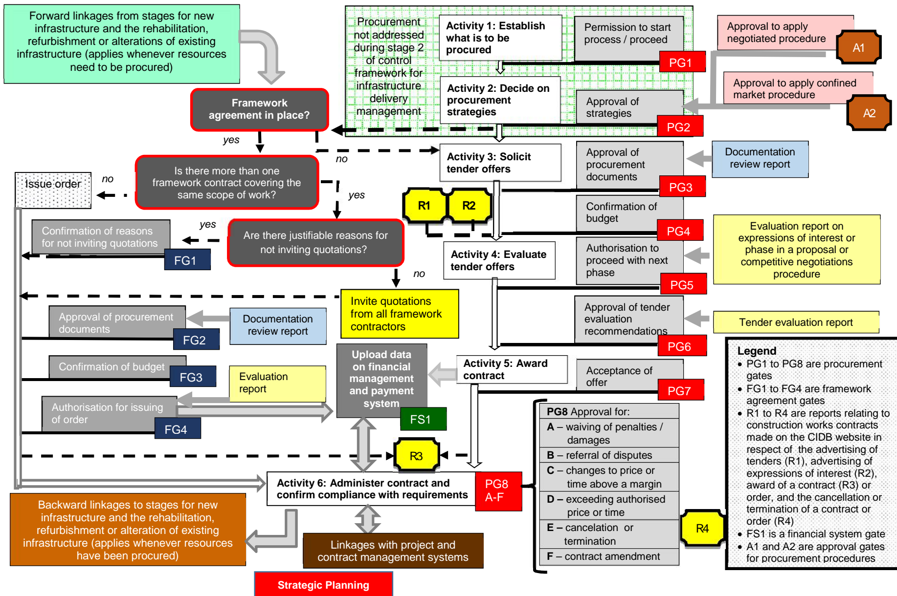
Control framework for infrastructure procurement
