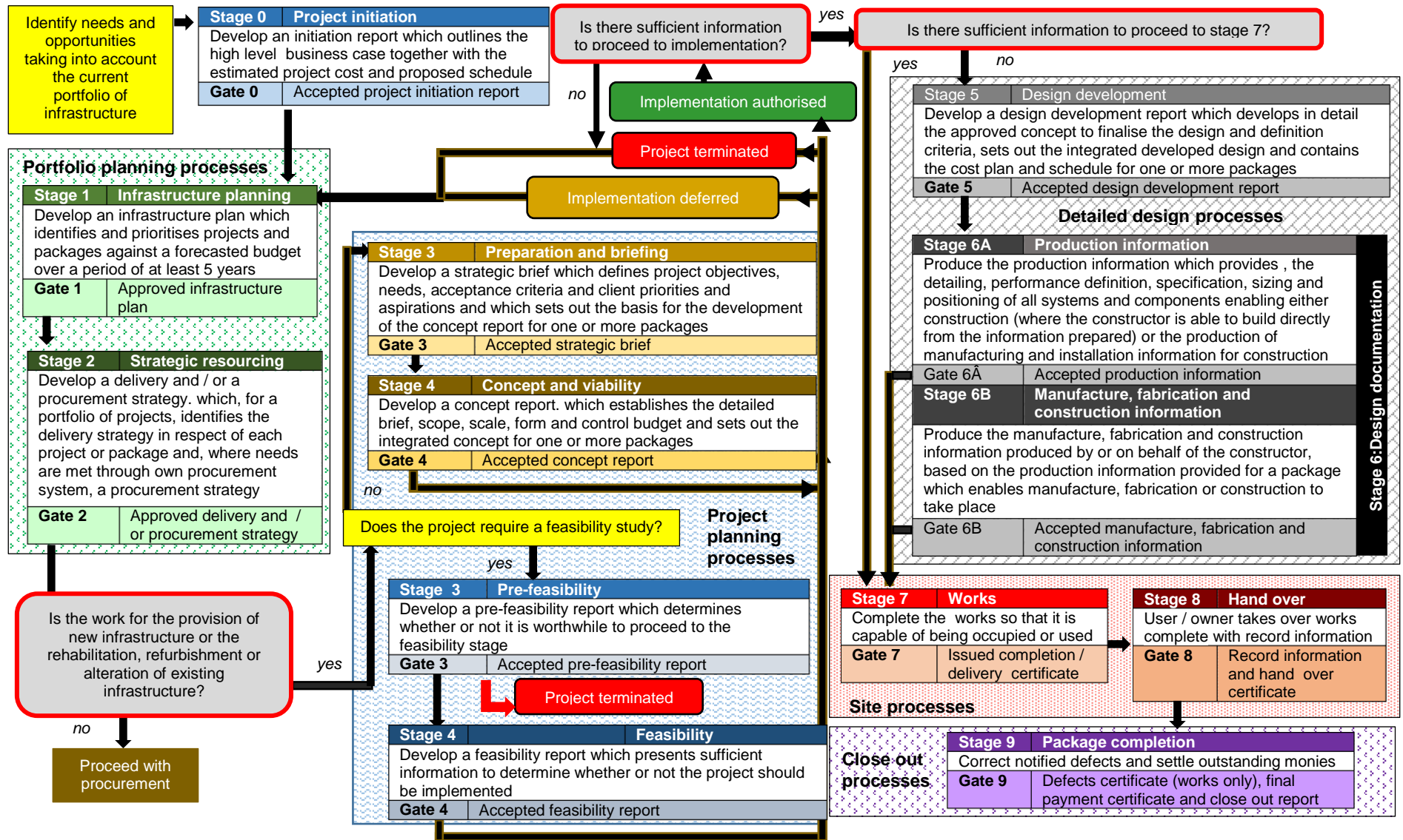
Control framework for the planning, design and execution of infrastructure projects
